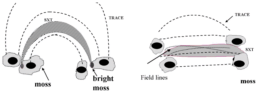
Figure 3. Graphical representation of the spatial relationship between the TRACE and the SXT loops in NOAA AR 8844
