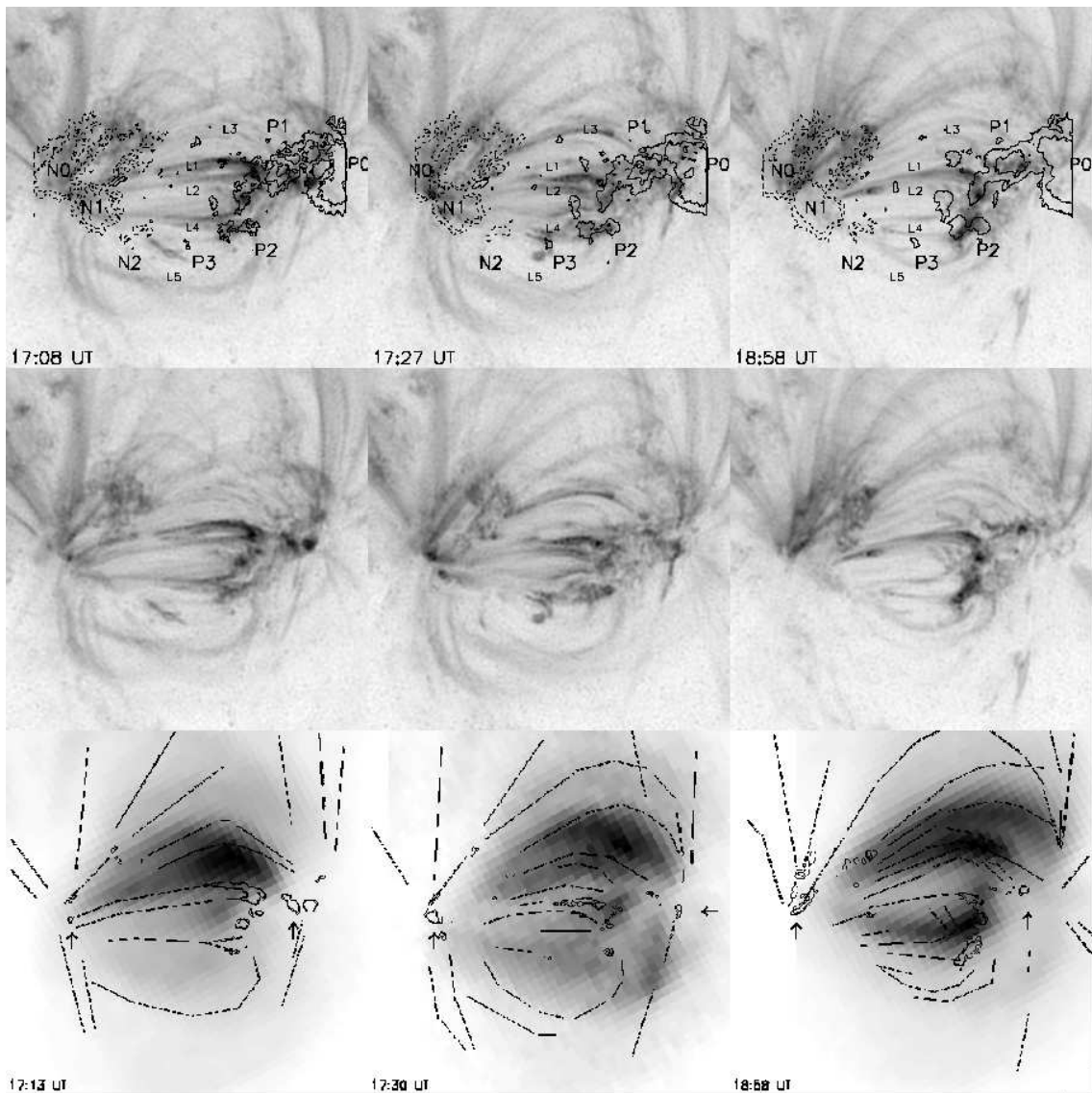
Figure 2. Co-alignment between the TRACE and the SXT loops: Upper row: Negatives of typical TRACE images taken at 171 \text{ \AA} . The first two images correspond to the first TRACE orbit, while that last image corresponds to the second TRACE orbit. The contours of the magnetic field strength are also shown, taken at 500 \text{ G} and at 1000 \text{ G} , while the labels of the magnetic polarities are given for reference. Solid/dashed contours indicate positive/negative polarity. The low-lying system of TRACE loops has been classified into five discrete loop sub-systems, labeled L1 to L5. Middle row: The same TRACE images without contours and labels. Lower row: Negatives of nearly simultaneous SXT images (taken within 5 \text{ min} from the TRACE observations) co-aligned with the shown TRACE images. The TRACE loops are represented by the dotted curves. The small contours indicated by the arrows correspond to brighter moss features, and they include the calculated locations of the SXT loop footpoints.
