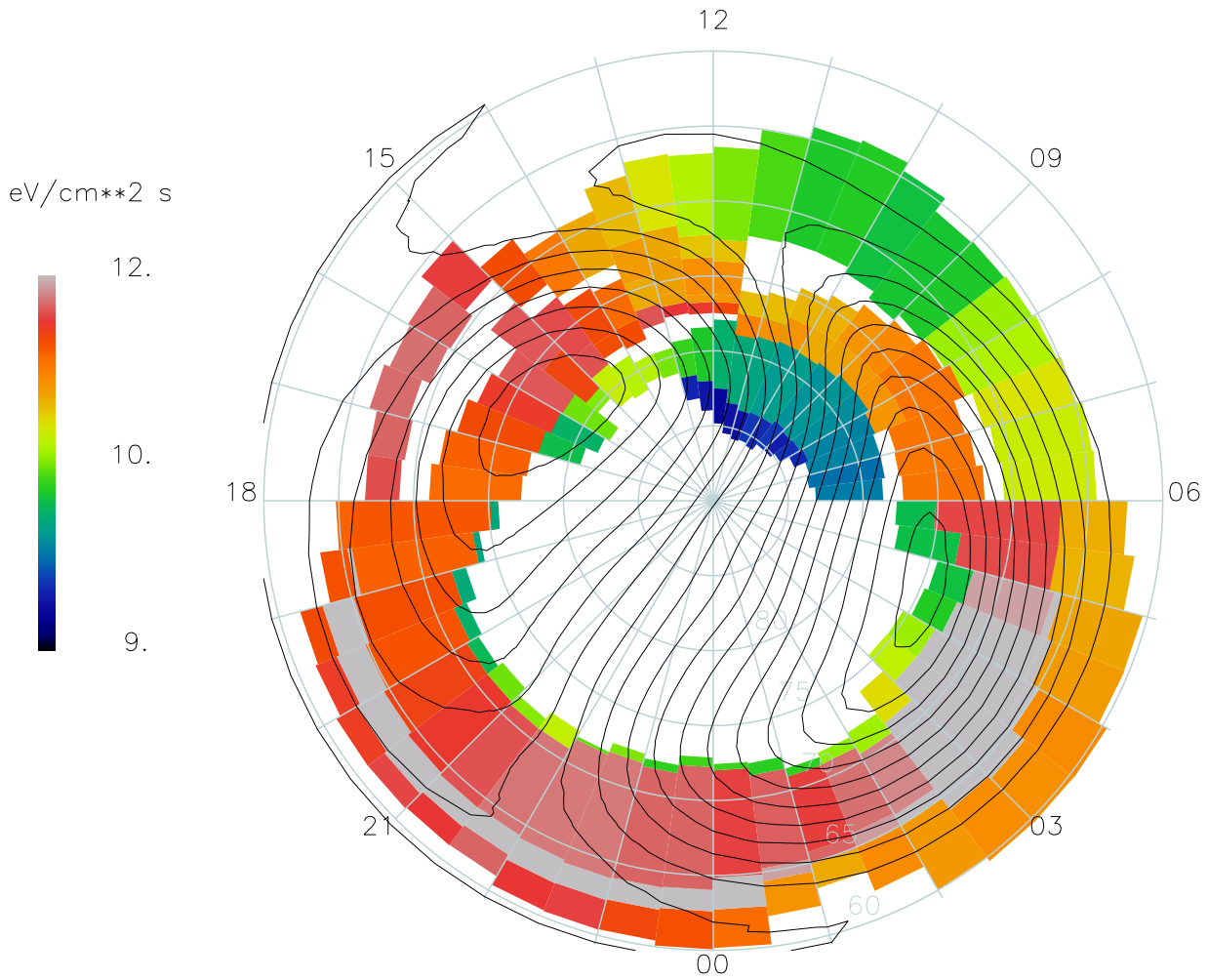
Plate 5. Same as Plate 1, except that ion energy flux (eV/cm 2 ) is plotted within region contours. (b) B_z < -1 , B_y > 3 nT
