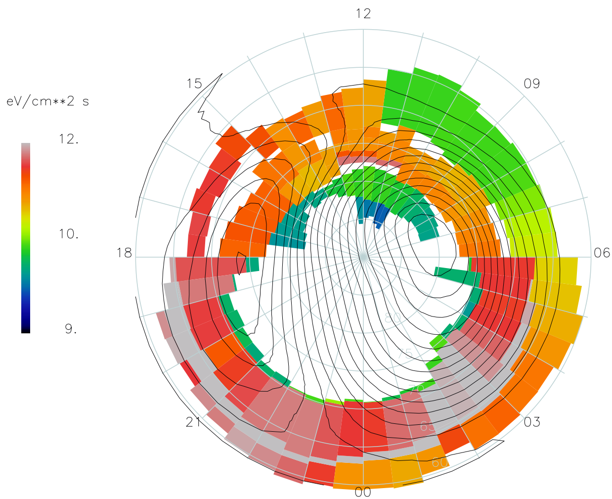
Plate 5. Same as Plate 1, except that ion energy flux (eV/cm 2 ) is plotted within region contours. (a) B_z < -1 , B_y < -3 nT
