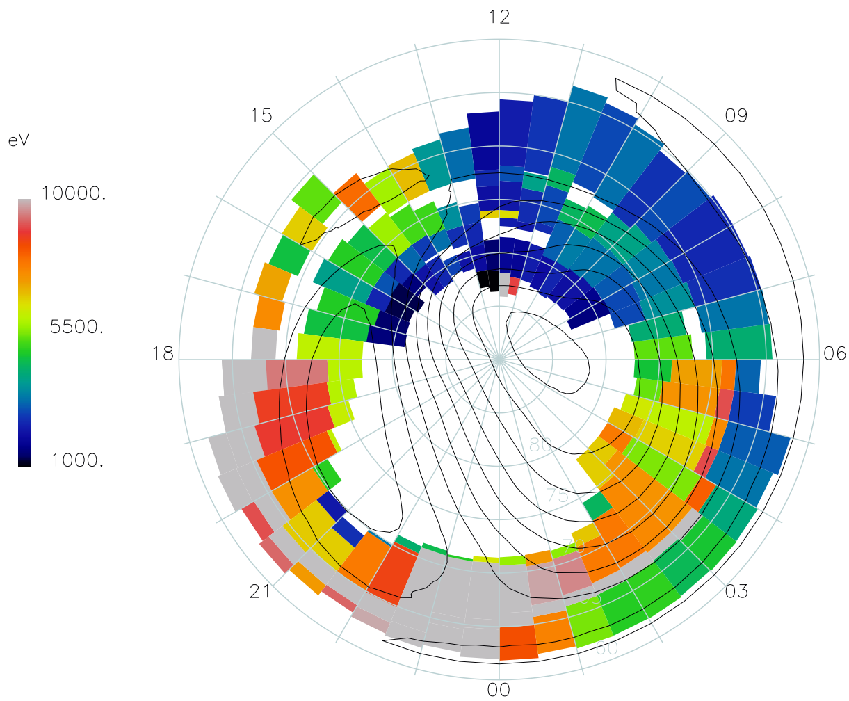
Plate 3. Same as Plate 1, except average ion energy (eV) is plotted within region contours. (c) B_z > 1 , B_y < -3 nT
