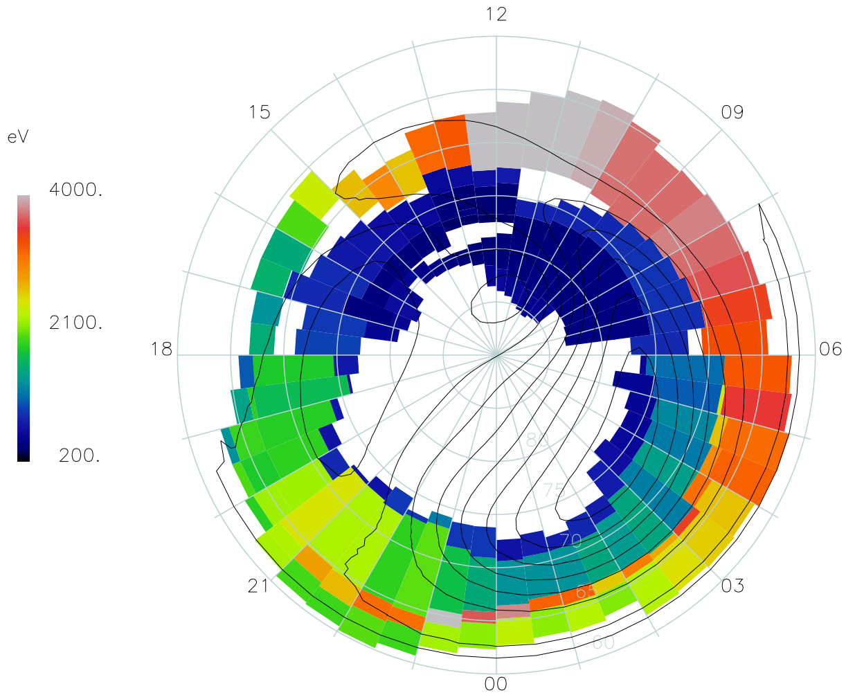
Plate 2. Same as Plate 1, except average electron energy (eV) is plotted within region contours. (d) B_z > 1 , B_y > 3 nT
