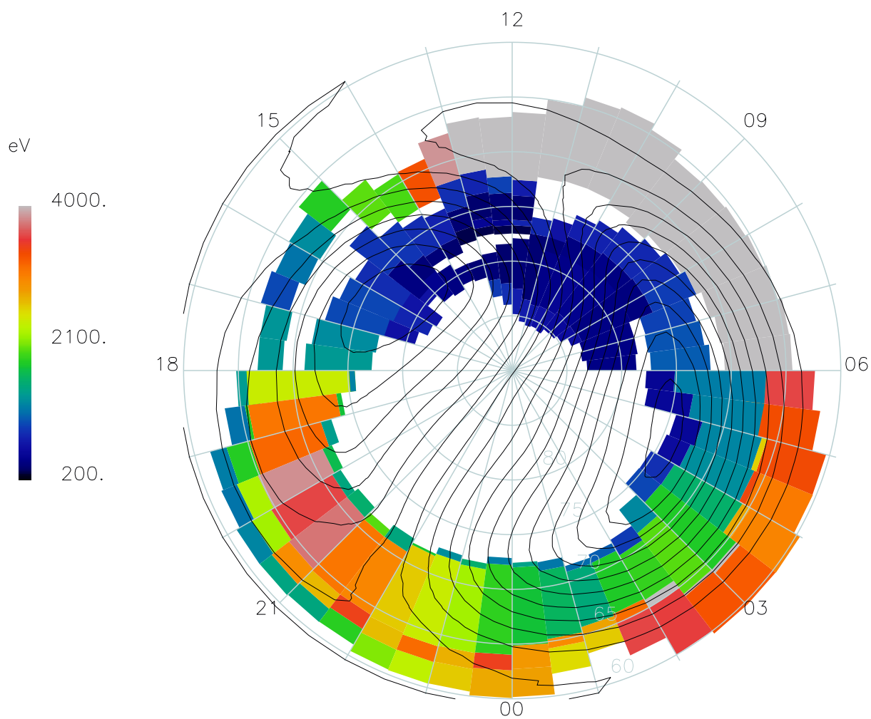
Plate 2. Same as Plate 1, except average electron energy (eV) is plotted within region contours. (b) B_z < -1 , B_y > 3 nT
